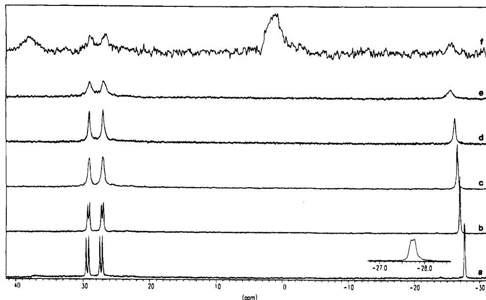
Figure 2. ^{31}\text{P}\{^1\text{H}\} NMR spectra (THF- d_8 , 81.01 MHz) of 3 recorded in the temperature range from 20 to 120 °C (traces a–e); for comparative purposes, trace a of Figure 1 is reproduced here as trace f.
