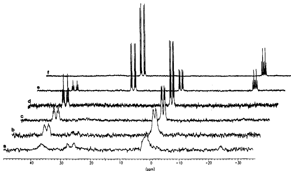
Figure 1. 31 P{ 1 H} HPNMR study (sapphire tube, THF- d 6 , 81.01 MHz) of the catalytic hydrogenation of BT in the presence of 1 (30 atm H 2 , substrate/catalyst ratio 100): after 4 h at 120 °C (a); (b–d) after the NMR probe was sequentially cooled to 100 (b), 80 (c), 20 °C (d); after the tube was depressurized to 1 atm of H 2 (20 °C, e); after all hydrogen was replaced by nitrogen (20 °C, f).
